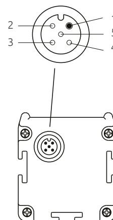
Emitter M12 5-pole Male
