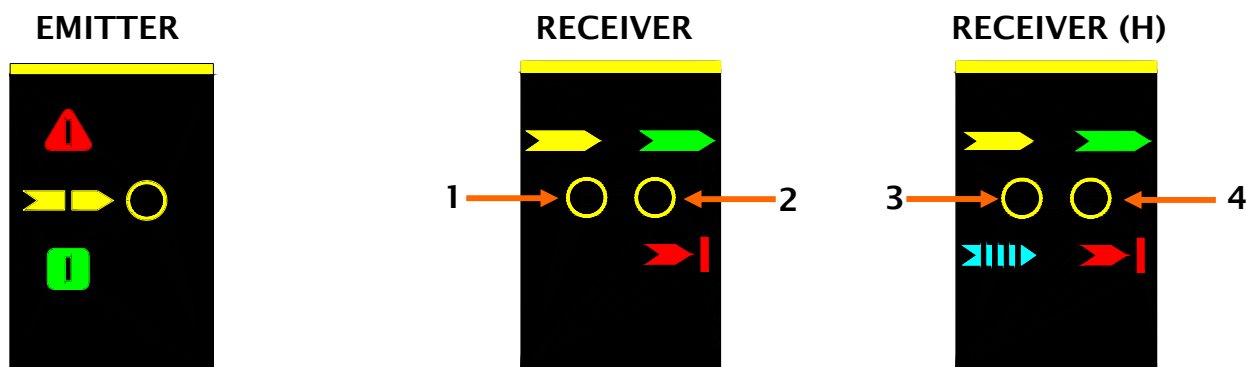
Figure 25 - Light signals
